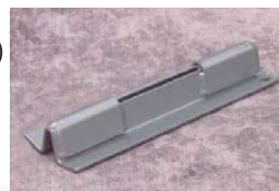
4048 Wide Draw Bar Overall Length: 14½" (368 mm) Width: 4" (102 mm) Weight: 7 lbs (3.18 kg) Capacity: 3 tons (2,722 kg)
